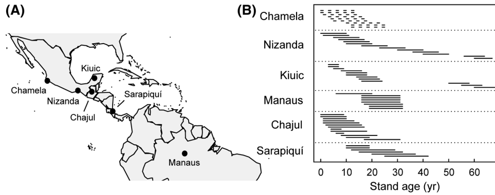
Figure 1. Geographic location and range of stand ages of the second-growth forests in each study site. A Map with the location of the six study sites. B Stand age range over which biomass dynamics were monitored for each site; each horizontal line represents the age range for a single plot. Plots in Chamela were monitored over 3-year intervals, plots in the other study areas were monitored at annual intervals.
