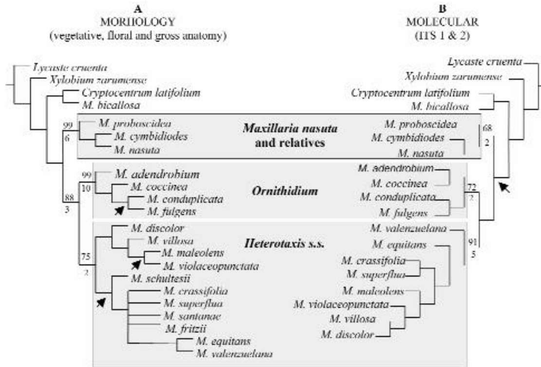
Figure 1. Consensus trees of phylogenetic relationships of Heterotaxis complex, A - based on morphological characters (morphology and gross foliar anatomy), and B - DNA sequences of internal transcribed spacers (ITS 1 & 2). Numbers above branches represent jackknife values, and numbers below branches Bremer support values. Nodes with arrows represent collapsed clades in the jackknife tree.
