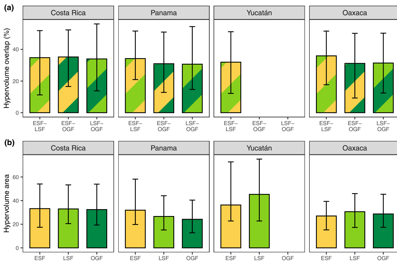
FIGURE 3 (a) Mean overlap statistics and (b) mean areas of the two-dimensional hypervolumes representing the ranges of demographic strategies for all successional stages (ESF, early successional forest; LSF, late successional forest; OGF, old-growth forest). Colored bars represent the median rarefied and bootstrapped values, error bars represent 95% confidence intervals ( r = 100 replicates, n = 10 species per successional stage). All values are means across pairs of demographic rates. Individual values per pair of demographic rates are given in Appendix S1: Figures S10 and S11.
