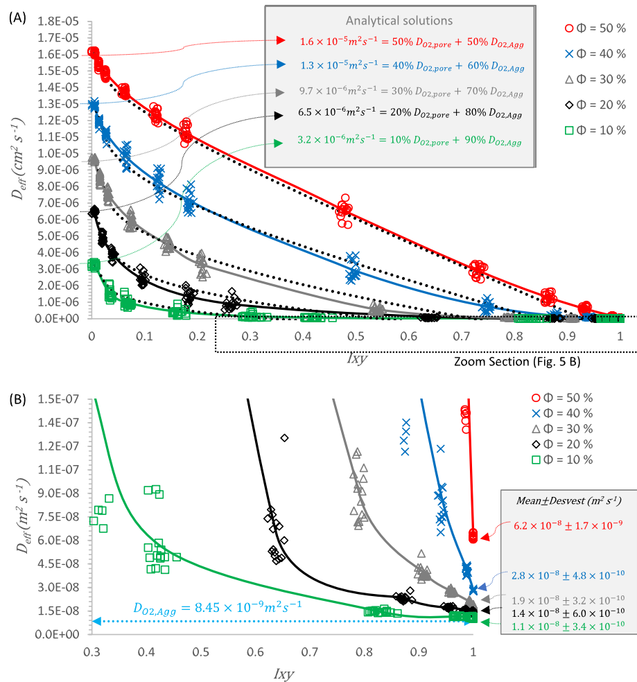
Figure 5. D_{\text{eff}} coefficient as a function of the isotropy evolution I_{xy} : (A) for all possibilities and analytical solutions magnitudes @ I_{xy} = 0 and (B) for a zoom section and numerical results @ I_{xy} = 1 .
