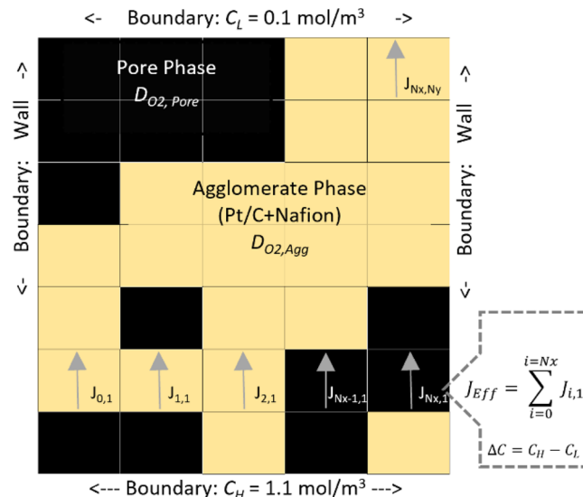
Figure 2. FVM boundary conditions and graphical index of the local fluxes used for the global \mathcal{J}_{eff} .
