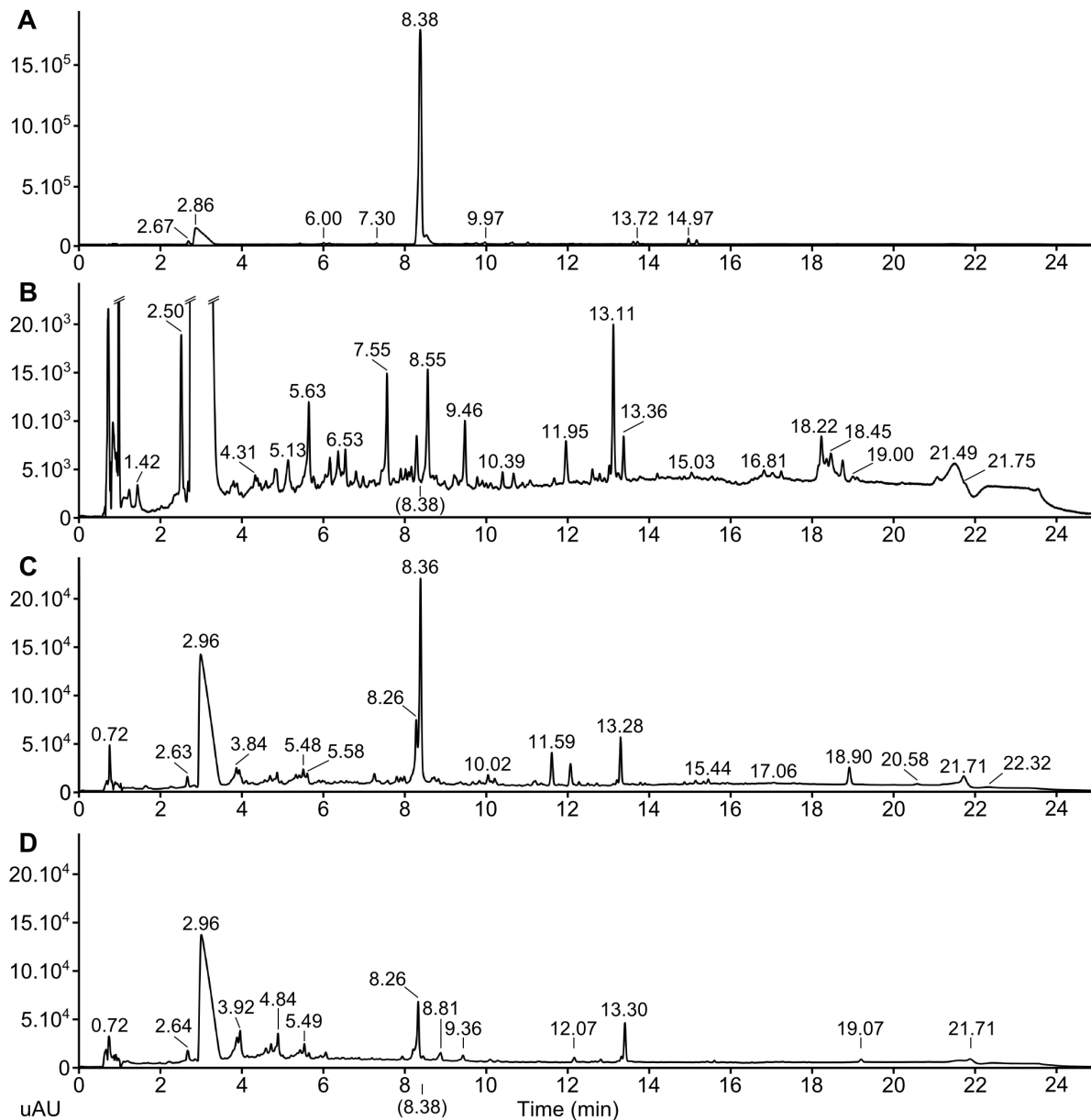
Figure 3. UHPLC detection of zinnin in fungal extracts. UHPLC chromatograms were obtained from different FRA017 Alternaria dauci fungal extracts and compared with an UHPLC chromatogram of pure synthetic zinnin. Retention times corresponding to main peaks are indicated A: UHPLC chromatogram of 10 \mu\text{g} synthetic zinnin. Observed zinnin retention time is 8.38 minutes B: UHPLC chromatogram of 13.4 \mu\text{g} organic extract of an A. dauci culture after 48 h under shaking conditions in carrot juice medium. Zinnin expected retention time of 8.38 minutes is indicated. C: UHPLC chromatogram of 13.4 \mu\text{g} organic extract of an A. dauci culture after 12 days without shaking (anoxic conditions) in V8 medium. A strong peak is visible, corresponding to zinnin retention time. D: UHPLC chromatogram of 13.4 \mu\text{g} organic extract of an A. dauci culture after 48 h under shaking conditions in V8 medium. Zinnin expected retention time of 8.38 minutes is indicated. Chromatograms C and D have the same scale. uAU: micro Absorption Units (optical density) at 233 nm. doi:10.1371/journal.pone.0101008.g003
