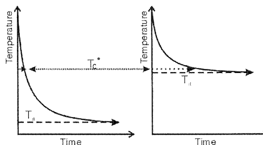
Figure 6 Scheme of the DSC oven cooling at: (A) T_{it} well below the onset of crystallization and (B) T_{it} at the onset of crystallization. The dotted line represents the T_c^* and the dashed line represents the T_{it} .
